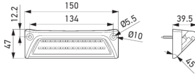
Dimensional sketch
